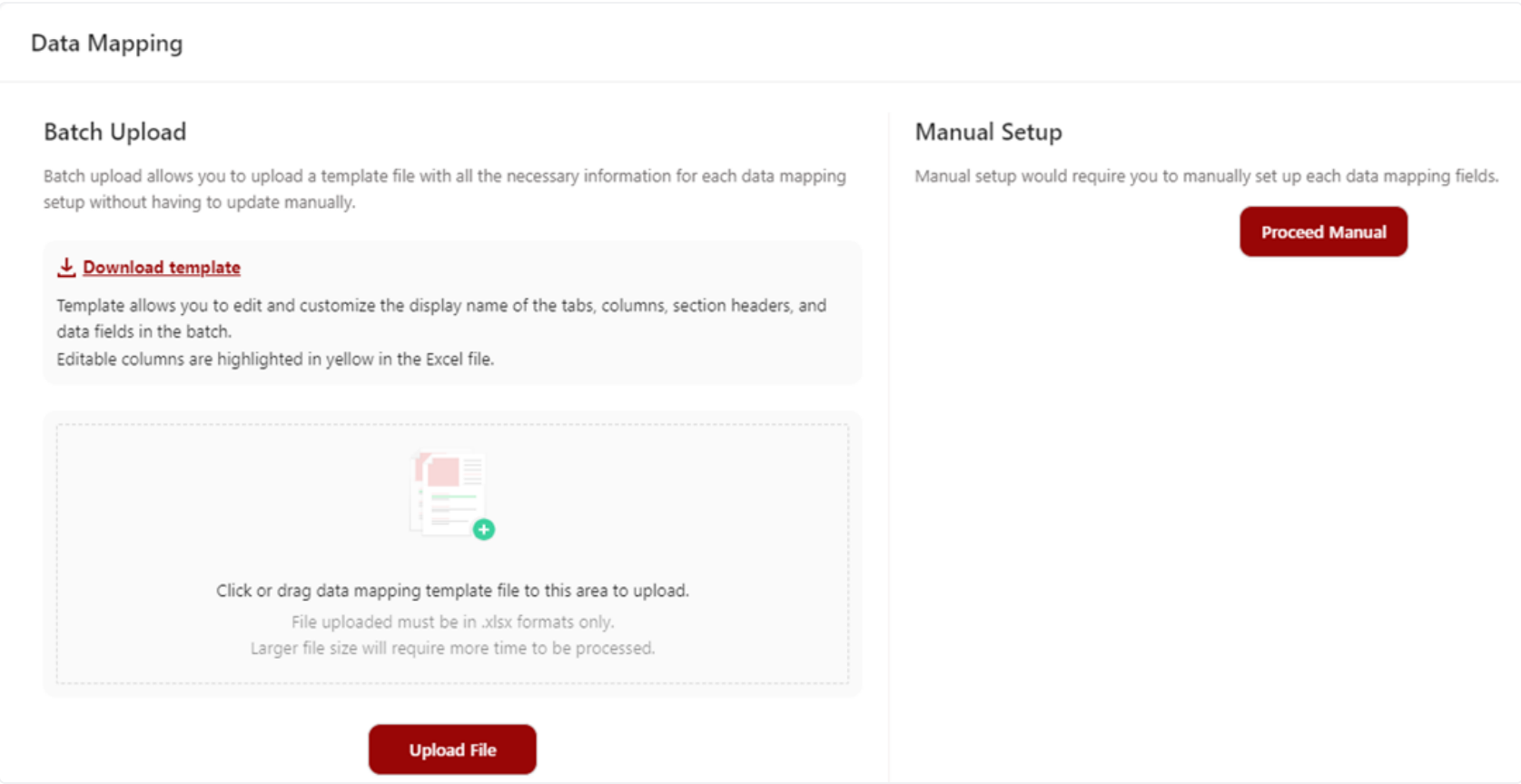
Figure 2.18: Data Mapping
