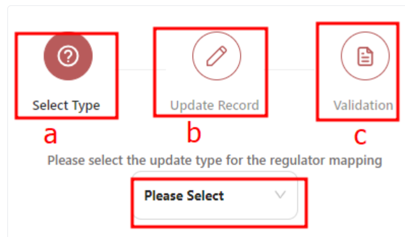
Figure 2.43: 3-Step Wizard
