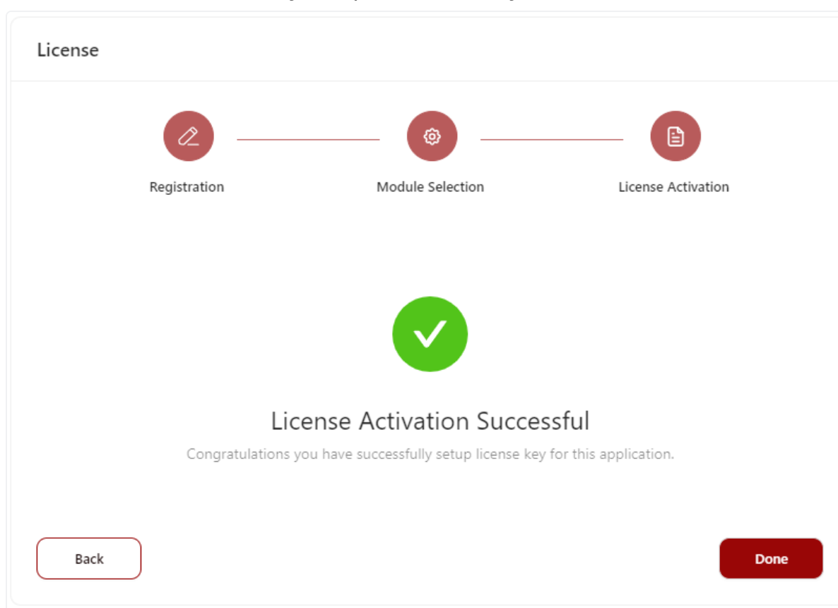
Figure 2.34: License Activation
